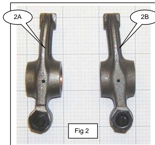
The Rocker Gear Assembly.
